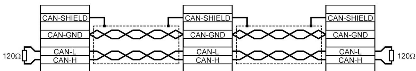
Figure 30: CAN bus cabling example
