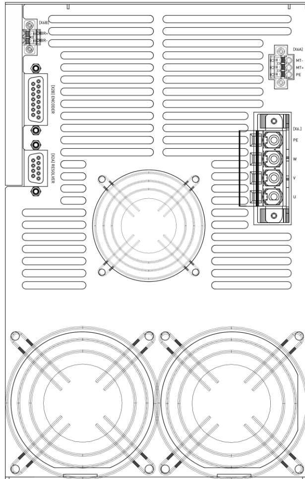
Figure 12: Servo drive ARS 2340 FS: Bottom view
