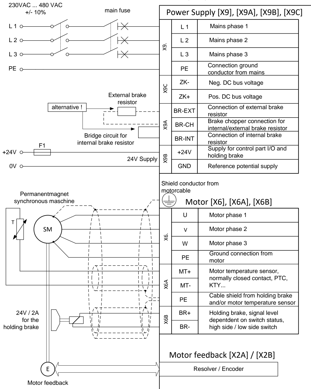
Figure 20: Connection to power supply [X9] and motor [X6]
