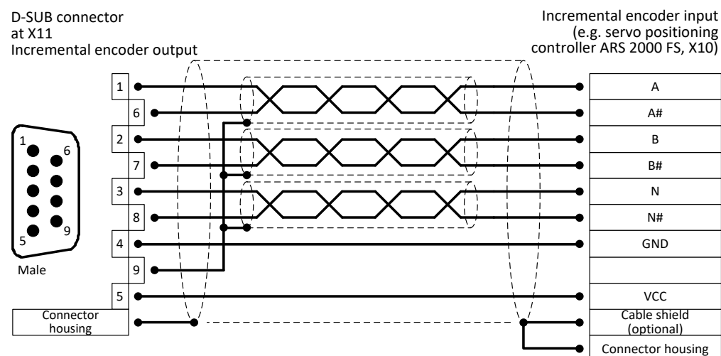
Figure 34: Pin assignment: Incremental encoder output [X11]
