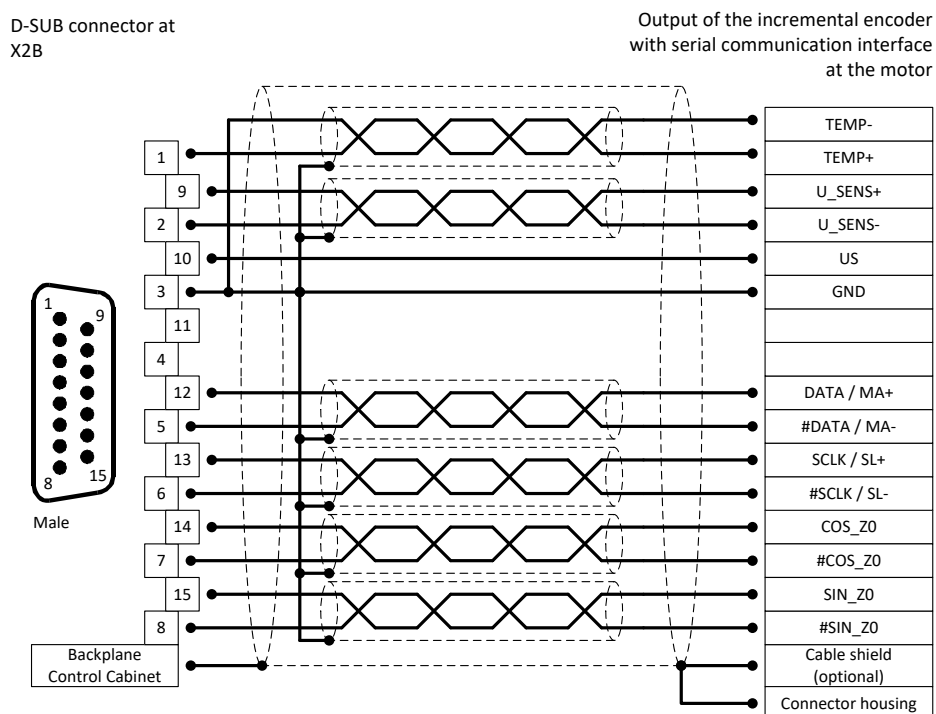
Figure 27: Pin assignment: Analog incremental encoder [X2B]
