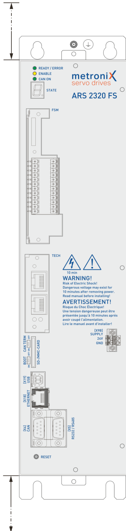
Figure 6: Servo drive ARS 2320 FS: Front view and Installation space
