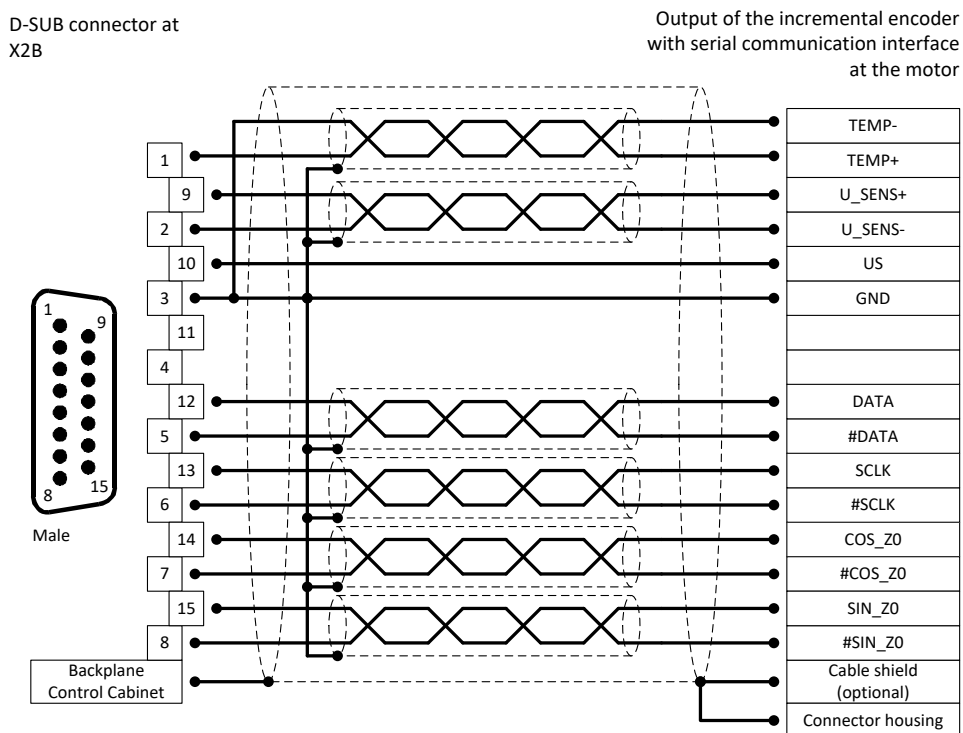
Figure 28: Pin assignment: Incremental encoder with serial communication interface (for example EnDat, HIPERFACE, BiSS) [X2B]
