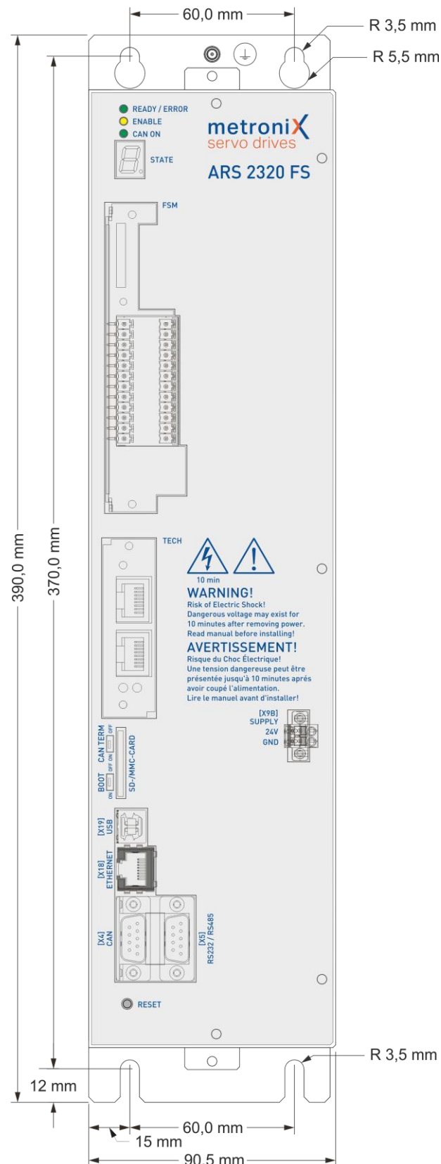
Figure 9: Servo drive ARS 2320 FS: Mounting plate
