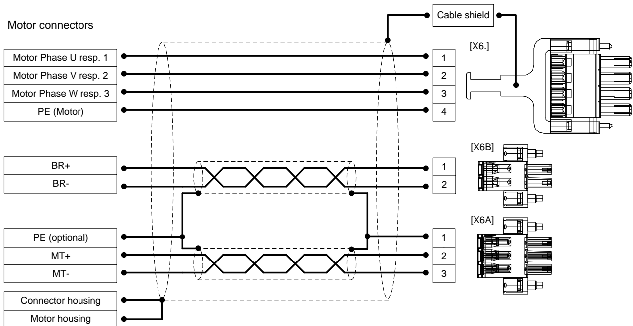
Figure 22: Motor connection [X6], [X6A] und [X6B]
