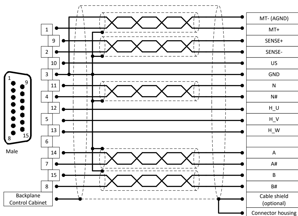
Figure 29: Pin assignment: Digital incremental encoder [X2B]
